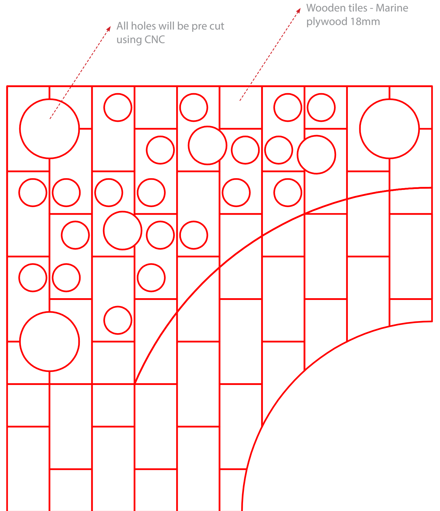
CLADDING - Wooden Tiles (18mm thickness)
