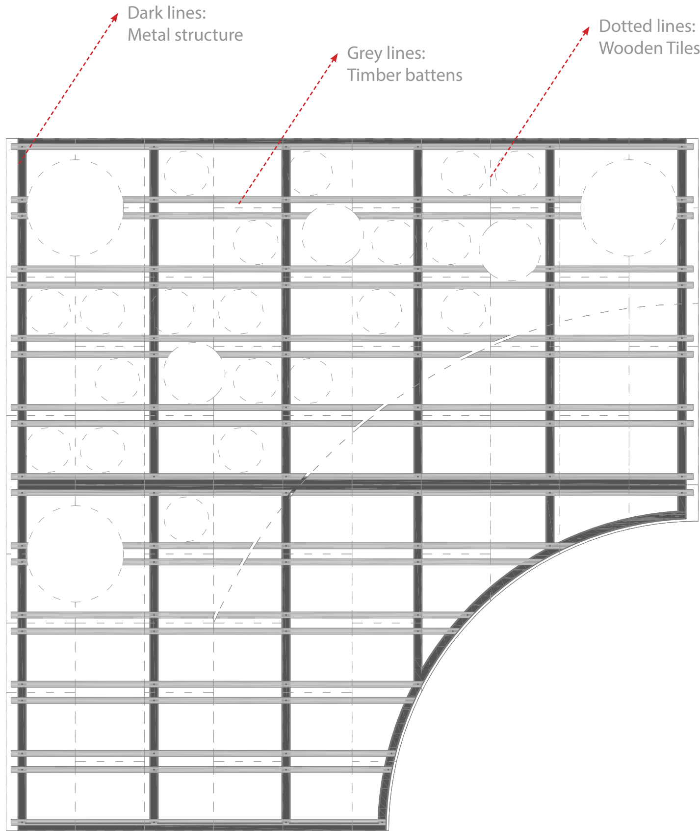
METAL STRUCTURE S AND TIMBER BATTENING
